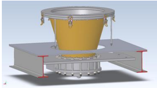
SolidWorks 3d engineering
