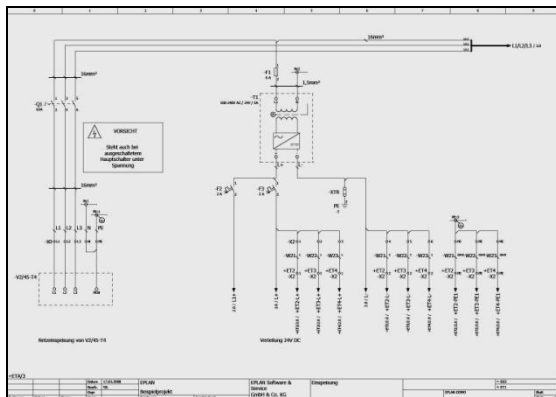
EPLAN P8 engineering
